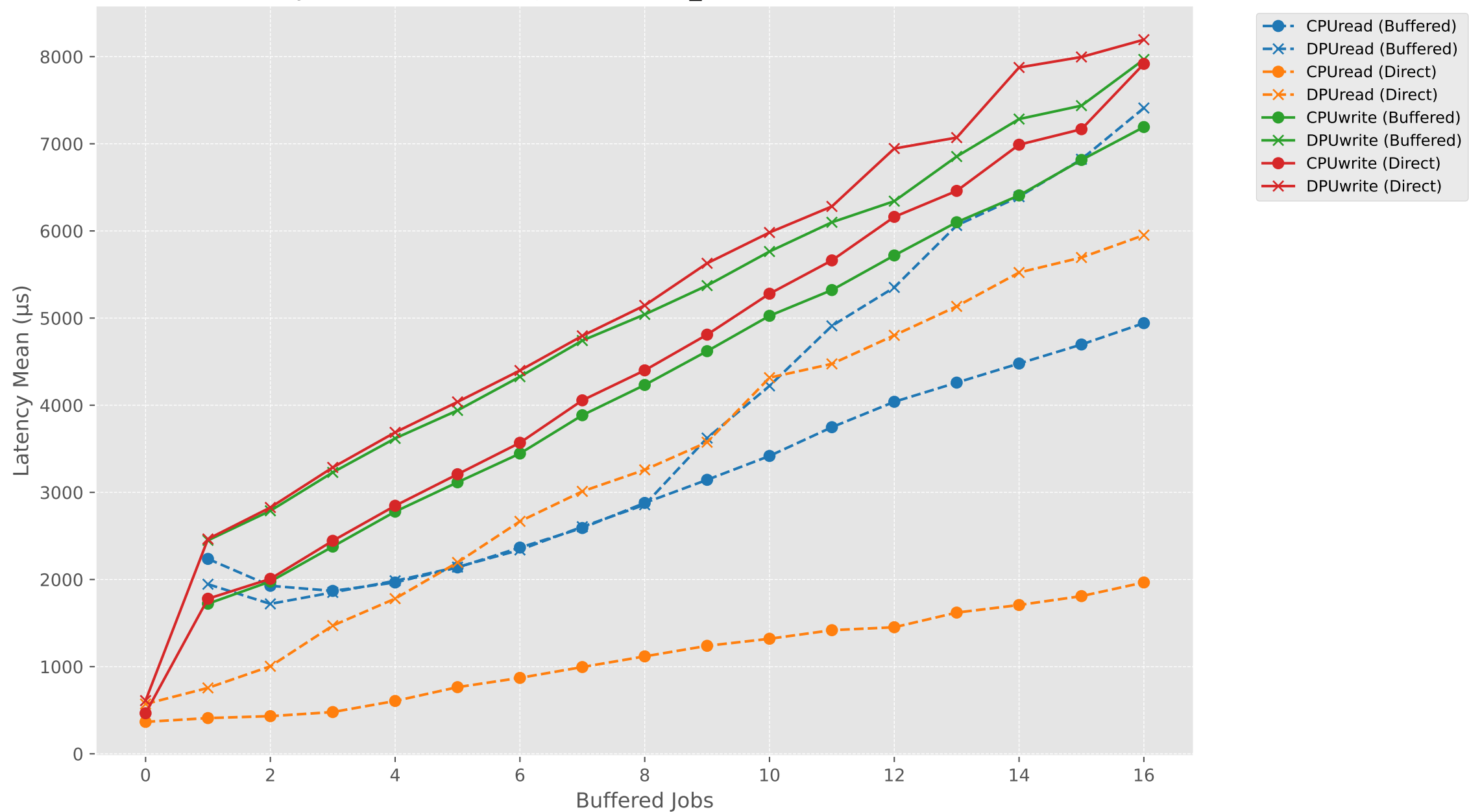
Latency Mean vs Buffered Jobs (direct1_bufferedN) - SEQ (CPU vs DPU)
